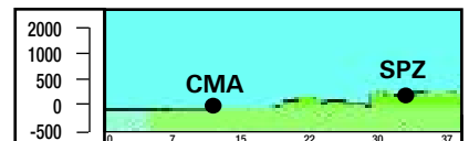
Profile map viewed from Camarillo Airport to Santa Paula Airport looking north
